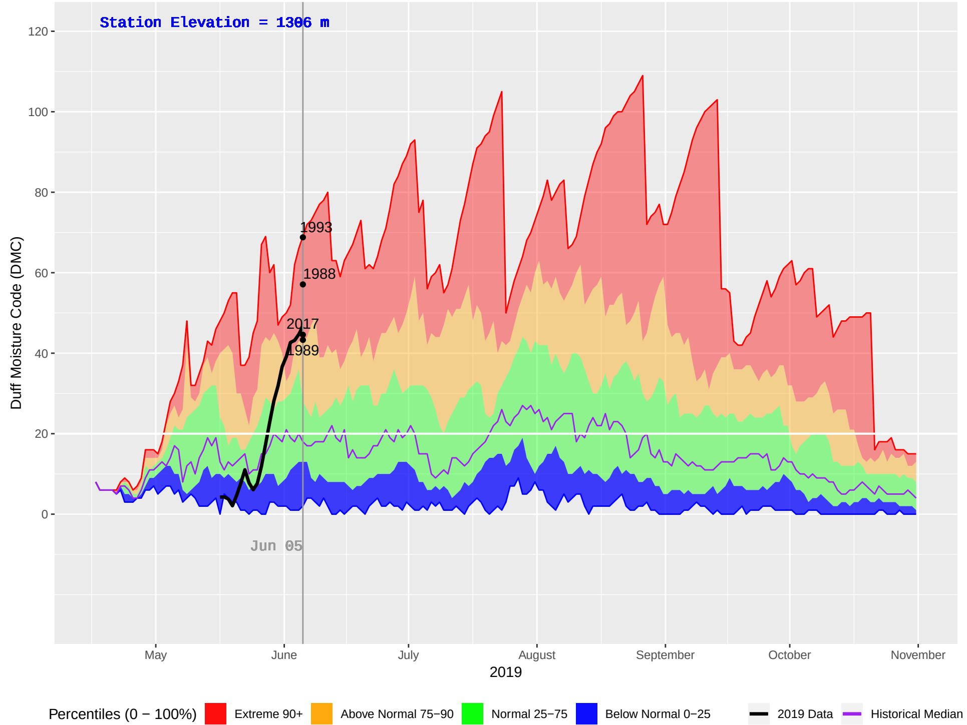
RED DEER (138) : Historical (1988–2018), Current (2019) Daily Duff Moisture Code (DMC)
