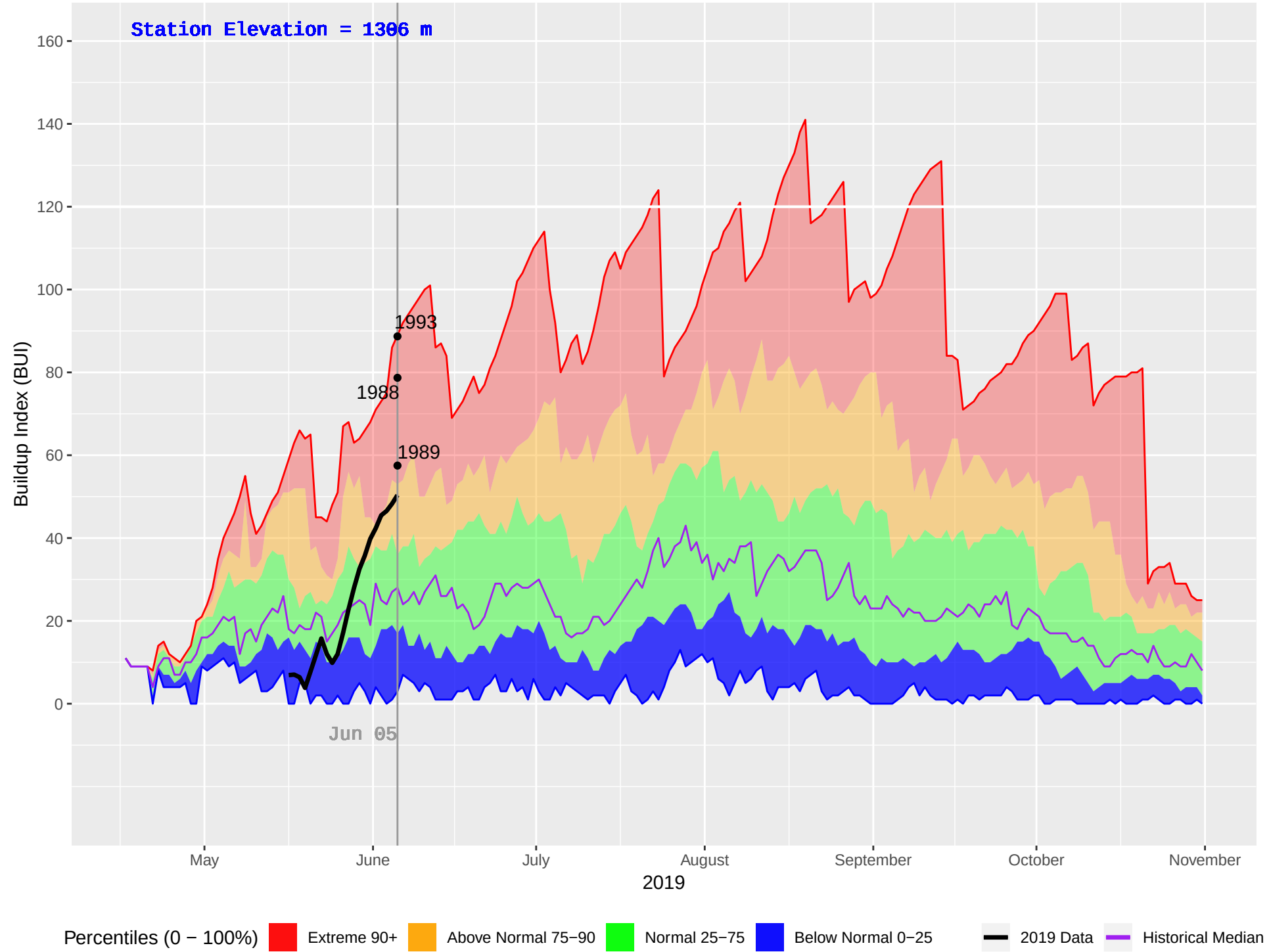
RED DEER (138) : Historical (1988–2018), Current (2019) Daily Buildup Index (BUI)
