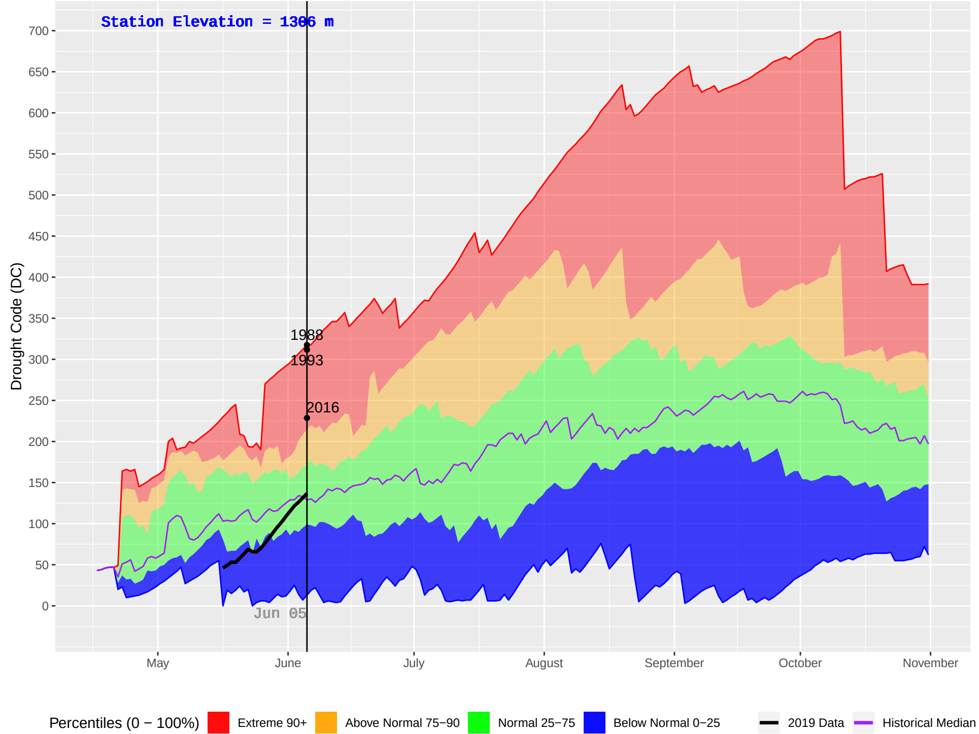
RED DEER (138) : Historical (1988–2018) and Current (2019) Daily Drought Code (DC)
