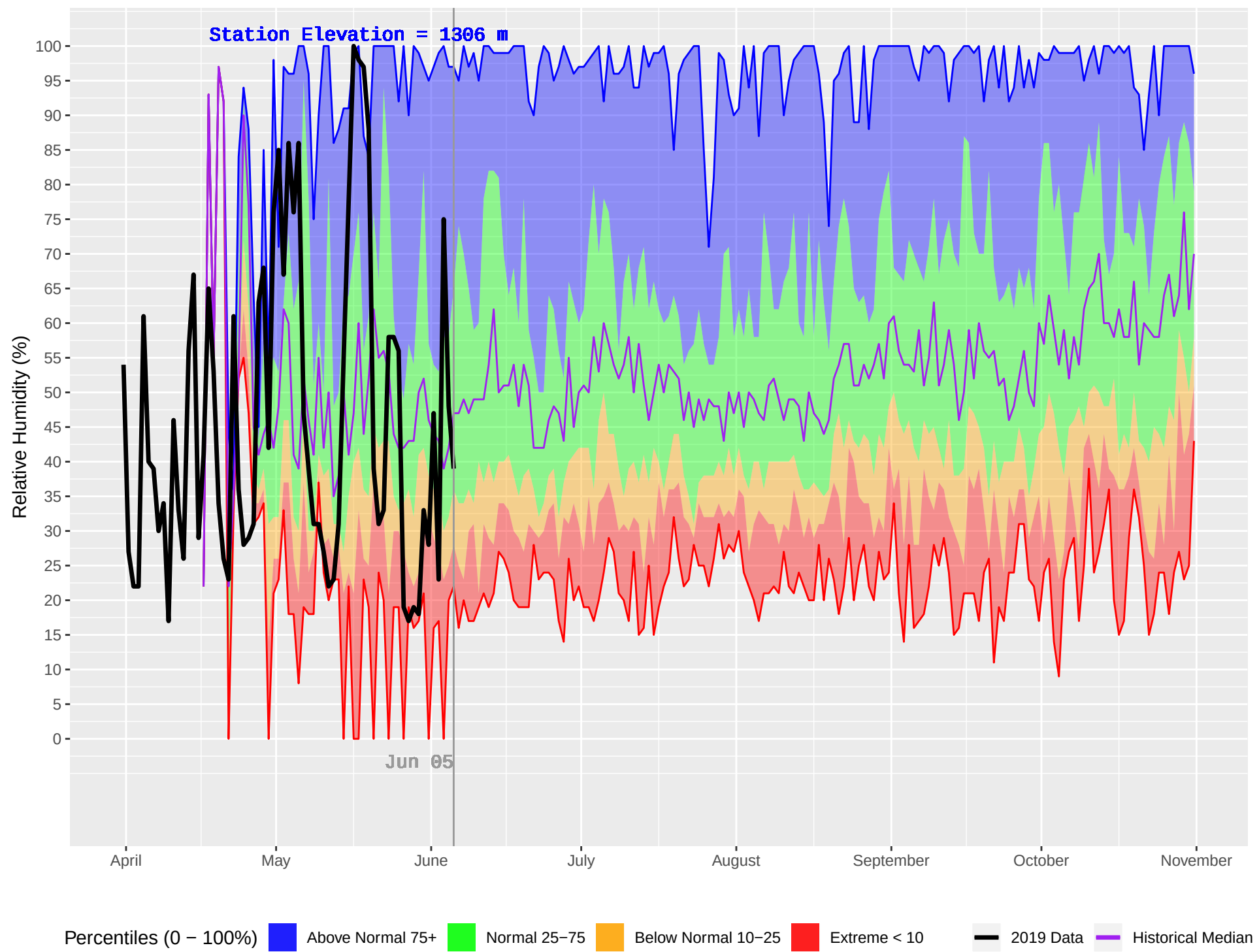
RED DEER (138) : Historical (1988–2018) and Current (2019) Daily Relative Humidity
