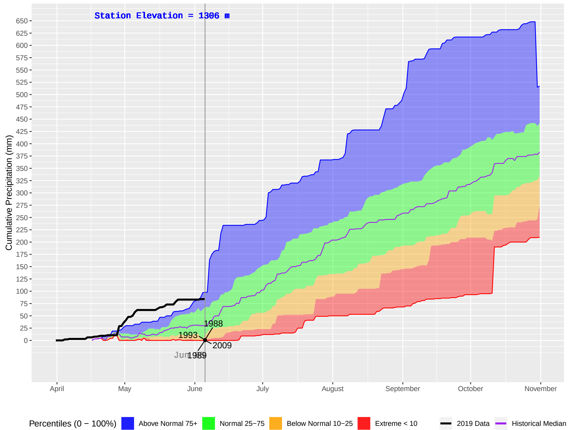
RED DEER (138) : Historical (1988–2018), Current (2019) Daily Cumulative Precipitation
